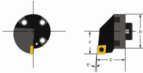
Positive 80° Diamond -5° Lead Coolant Thru
