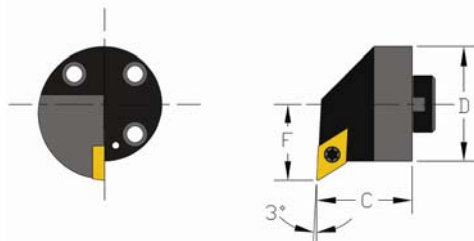
Positive 55° Diamond Profiling -3° Lead Coolant Thru
